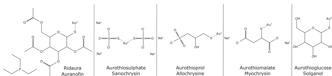
Fig. 1. Therapeutic gold salts structures and most common names. Structures have been drawn according to PubChem database ( https://pubchem.ncbi.nlm.nih.gov/ ).
