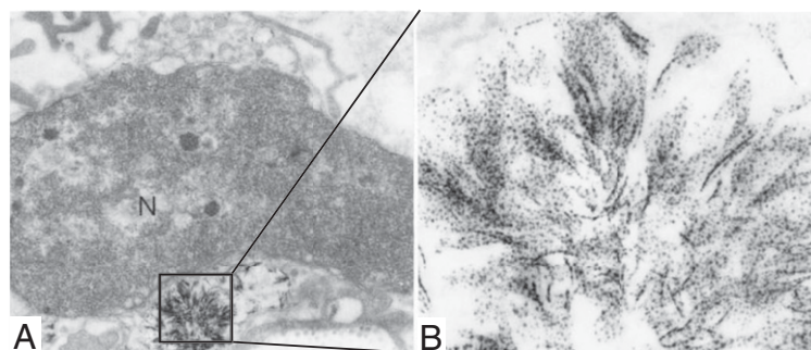
Fig. 2. (A and B) Aurosomes observed in patient's buttocks skin after chrysotherapy. Magnifications: (A) \times 12,000 ; (B) \times 136,000 . Reprinted by permission from ref. 44, Springer Nature: Archives of Dermatological Research , copyright (1990).
